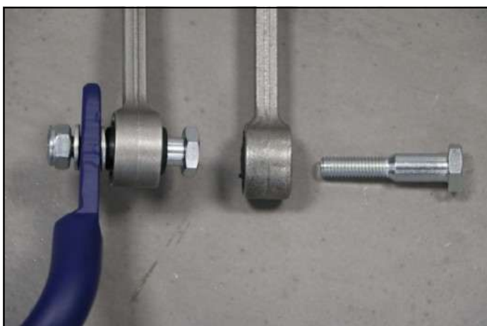
Fig. 1: Configuration for mounting of special screw
